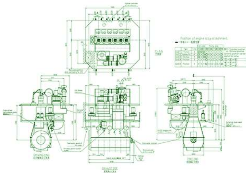
Outline arrangement
